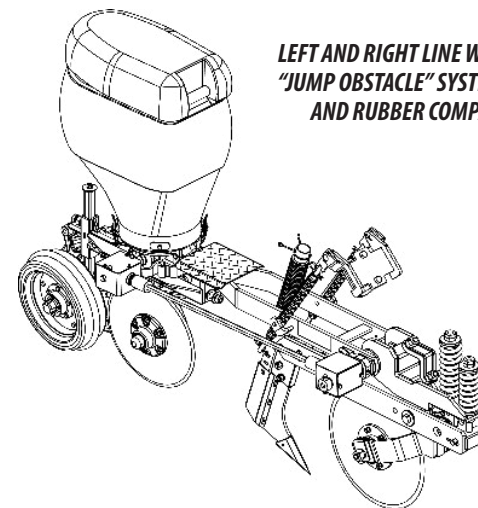
FERTILIZER CART WITH AND WITHOUT "JUMP OBSTACLE" SYSTEM W / FURROWER
