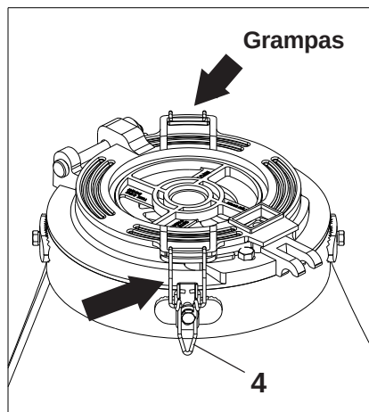
Detalle "E"
