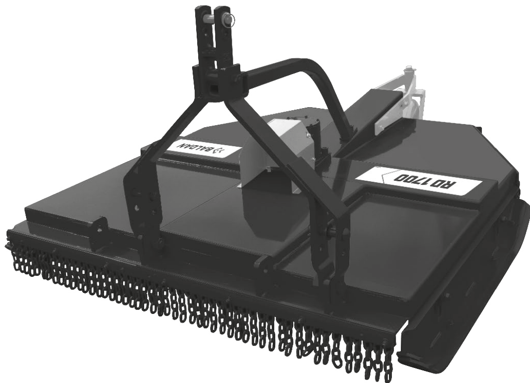
RD/RDU 1300/1500/1700 Roçadeira Hidráulica Central e Lateral
