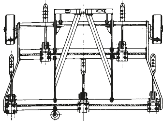
ASTH 9 x 5 Shanks
