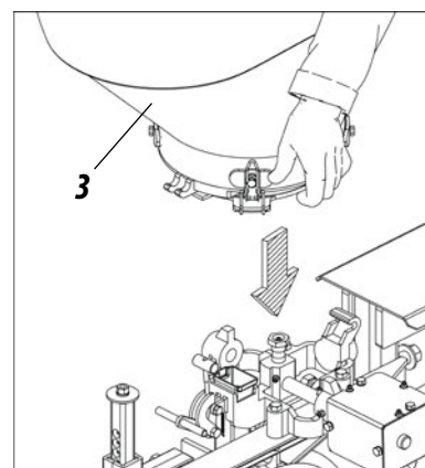
Detail "I"
