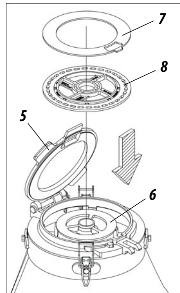
Detail "G"
