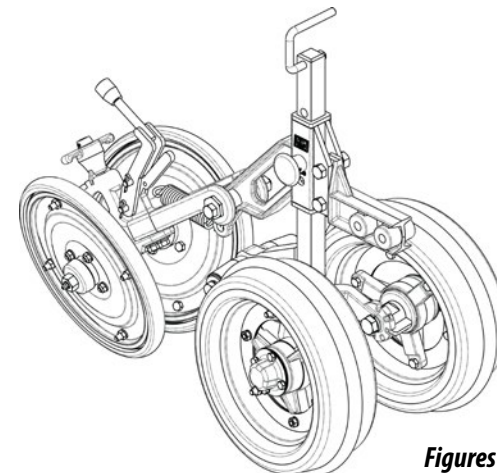
Oscillating eccentric depth wheel cart cpl Code: 5124010557-1
