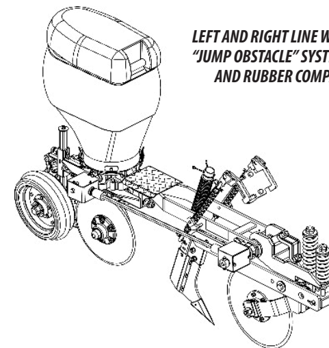
LEFT AND RIGHT LINE WITH AND WITHOUT "JUMP OBSTACLE" SYSTEM W / DISCO DOUBLE AND IRON COMPACTION WHEEL
