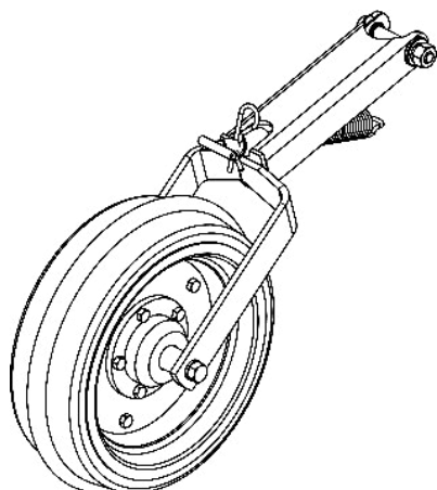
CONVEX COMPACTION WHEEL CART
