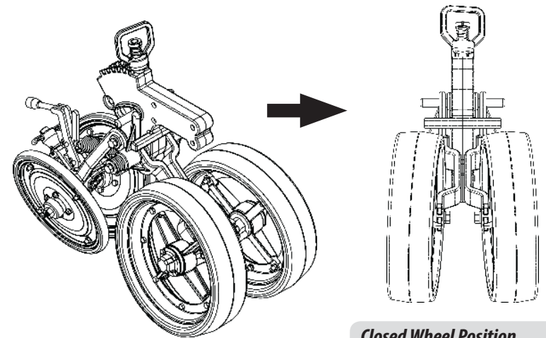
Closed Wheel Position
