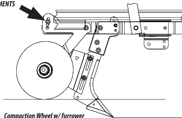
Compaction Wheel w/ furrower
