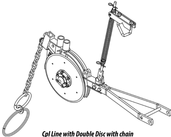
Cpl Line with Double Disc with chain Code: 2517011507-7
