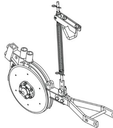
Cpl Line with Double Disc without chain Code: 5124010568-7
