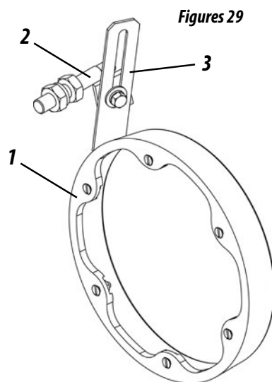
Right Depth Frame Cpl Code: 5288010047-5
