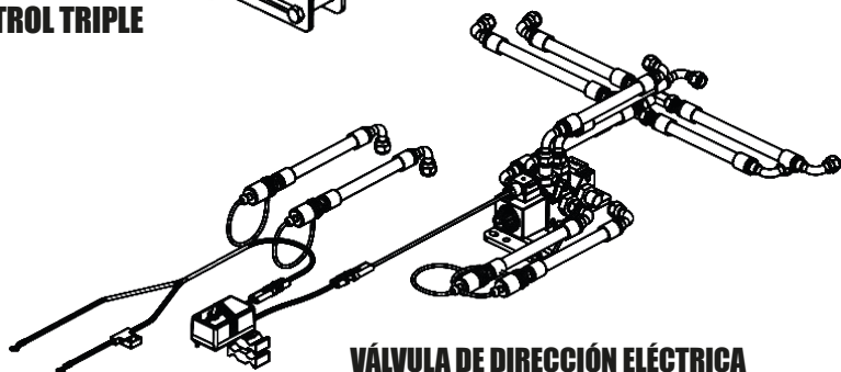
CONTROL TRIPLE
