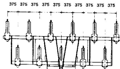
ASDA-MP 11 Hastes
