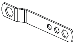
CHAVE P/ PORCA SEXTAVADA DE 1 1/4" - 1" - 3/4" E 5/8" NVCR
