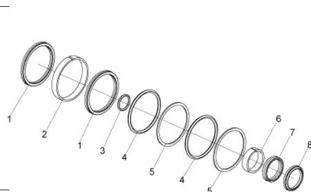
Sealing Kit LENIORS
