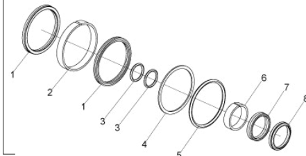
Sealing Kit MOCDROL
