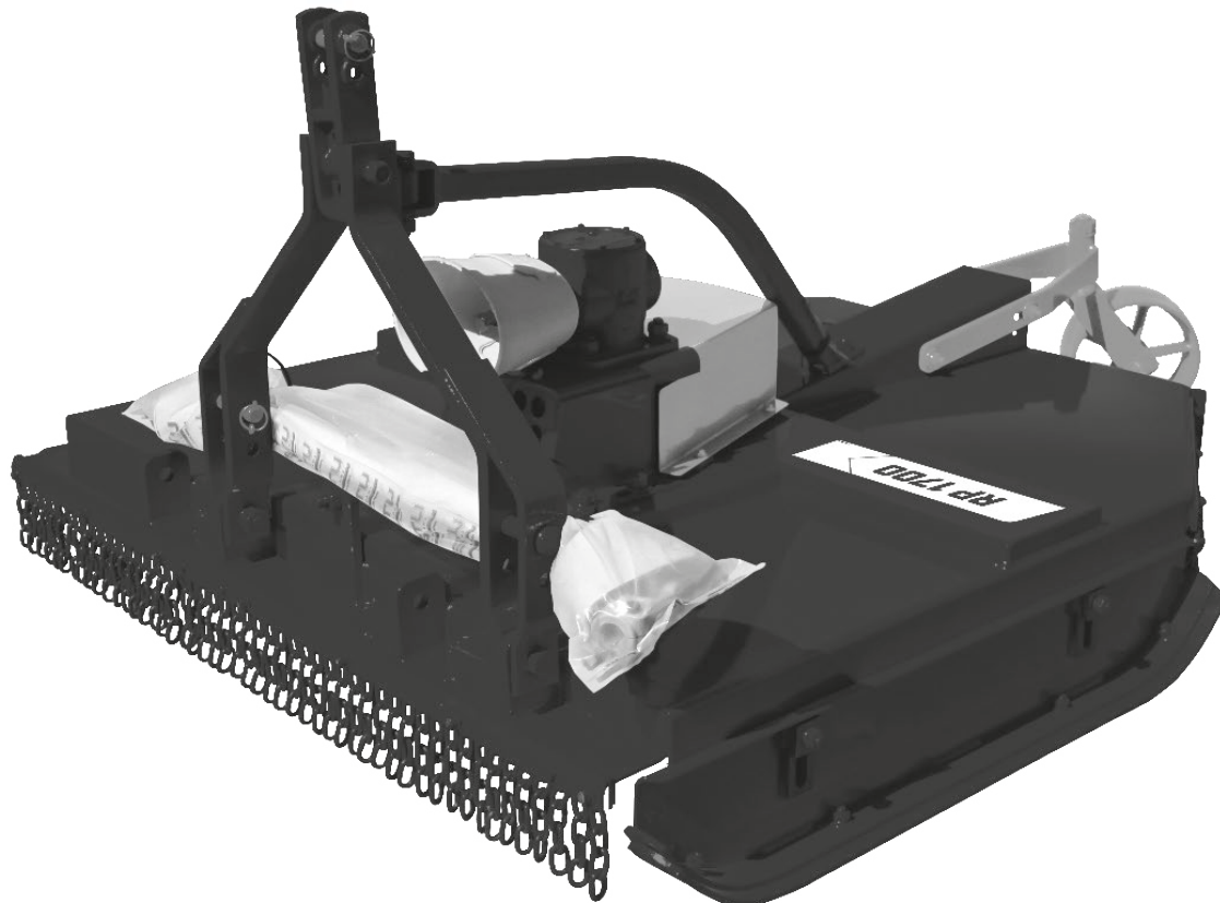
RP/RPU 1300/1500/1700 Central and Lateral Mounted Rotary Cutter
