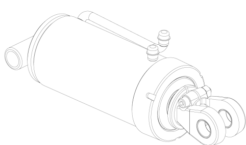
LENIORS Sealing Kit
