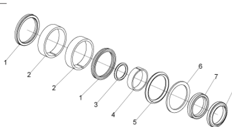
Sealing kit MOCRODOL
