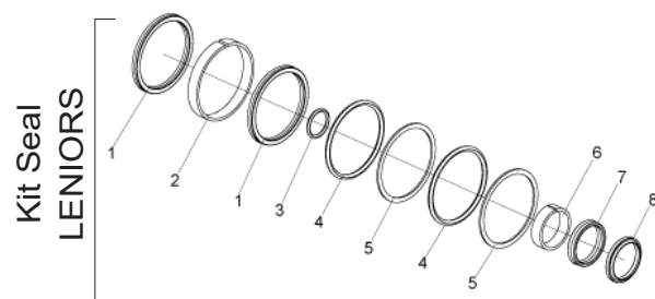
* Drawbar Lift Cylinder
