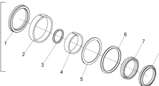
LENIORS Sealing Kit
