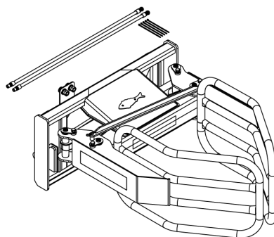
Bale Fork 5304010013-6 See page 55
