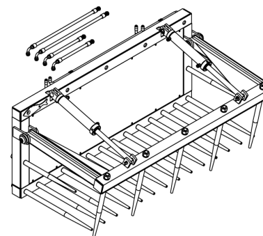
Silage Fork 2547260502-2 See page 56
